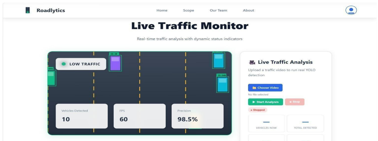
Fig 6.4.2 Analysis page
